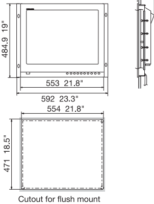
Cutout for flush mount
