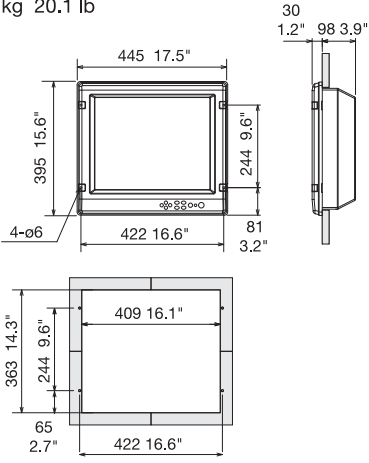
Cutout for flush mount
